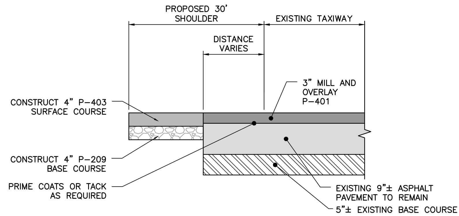
5 C-5 TYPICAL TAXIWAY SHOULDER NTS
