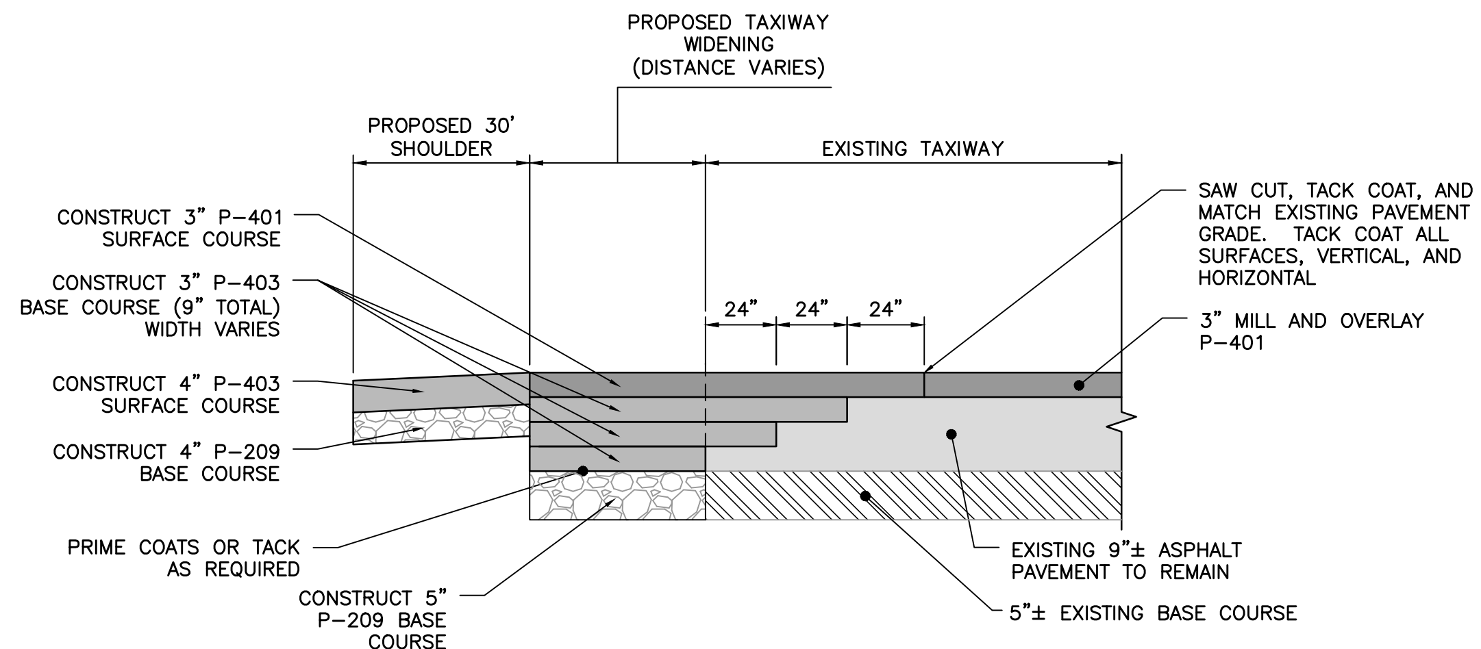
6 C-5 TAXIWAY A AND B2 WIDENING NTS
