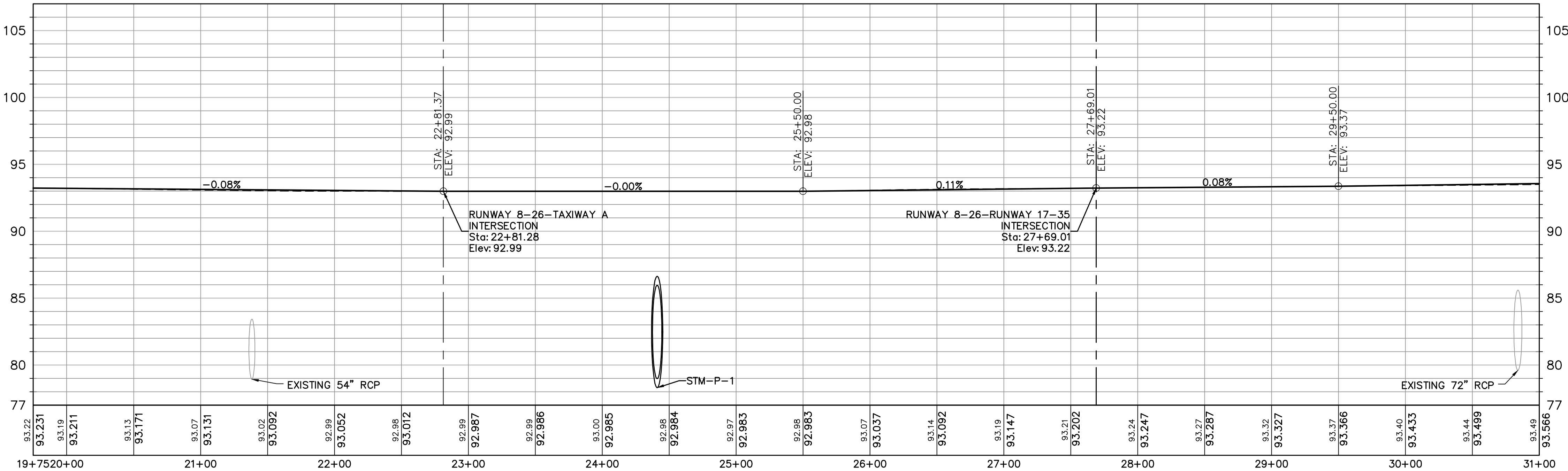
RUNWAY 8-26 HORIZONTAL SCALE: 1" = 50' VERTICAL SCALE: 1" = 5'
