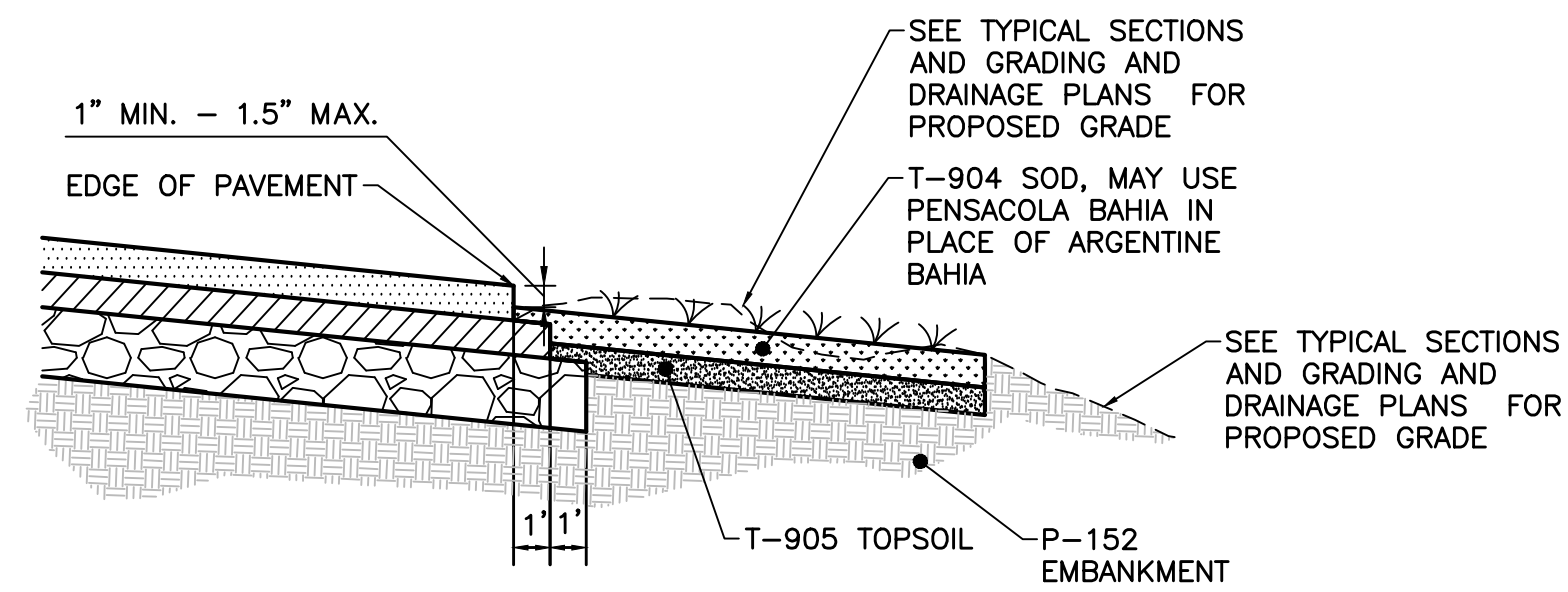
4 C-5 EDGE DROP OFF DETAIL - EOP TO TURF NTS
